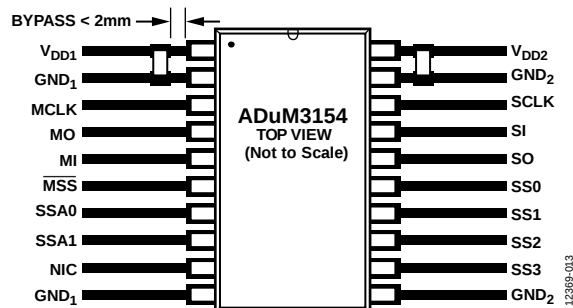
Figure 13. Recommended PCB Layout
