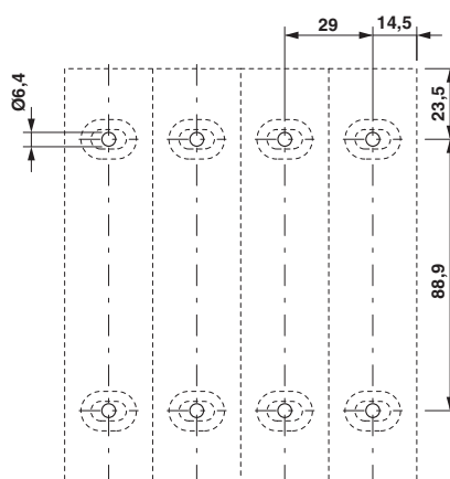
Dimensional drawing
