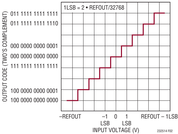
Figure 2. LTC2325-14 Transfer Function
