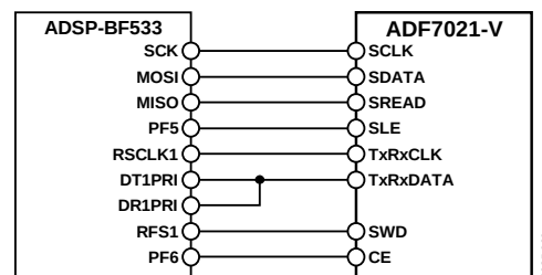
Figure 61. ADSP-BF533 to ADF7021-V Connection Diagram
