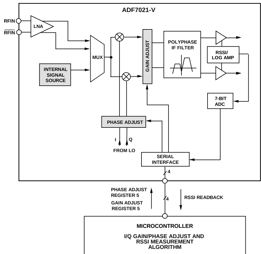
Figure 51. Image Rejection Calibration Using the Internal Calibration Source and a Microcontroller
