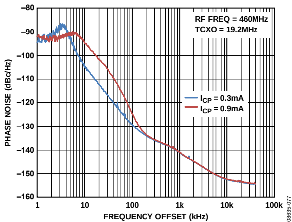
Figure 11. Phase Noise Response at 460 MHz, V_{DD} = 3\text{ V}
