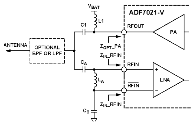
Figure 49. ADF7021-V with Internal Tx/Rx Switch
