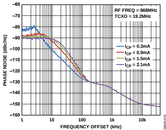
Figure 12. Phase Noise Response at 868 MHz, V_{DD} = 2.3\text{ V}
