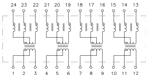
Circuit B
