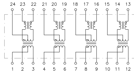
Circuit A
