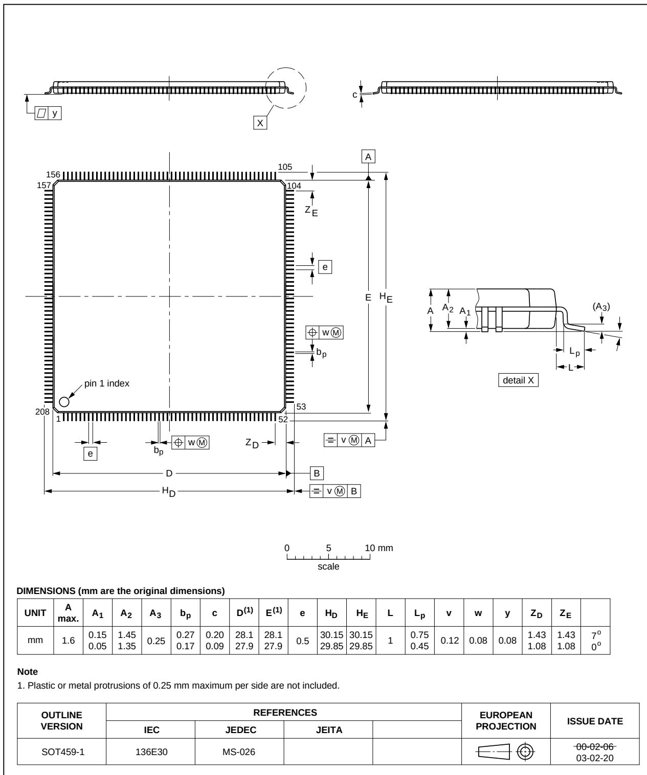
Fig 50. LQFP208 package
