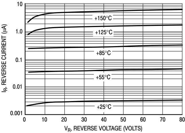
Figure 2. Reverse Current
