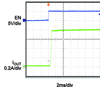
Short Circuit Current, Device Enabled into Short
