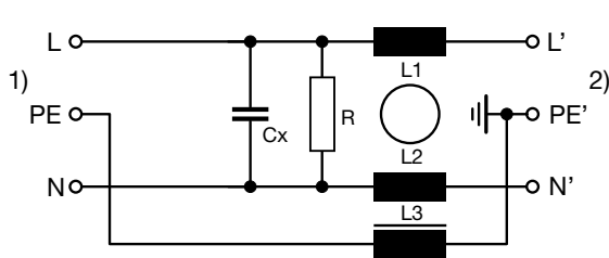
Medical Version (M5) with ground line choke
