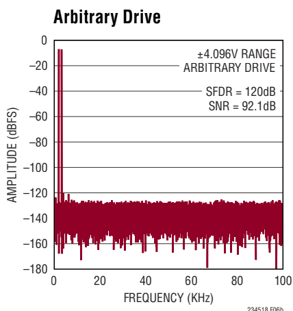
Figure 6b. Two-Tone Test. IN^+ = -7 dBFS 2kHz Sine, IN^- = -7 dBFS 3.1kHz Sine, Common Mode = 2.5V, 32k Point FFT, f_{SAMPL} = 200 ksps. Circuit Shown in Figure 6a with LT6237 Amplifiers, R_{FILT} = 40.2\Omega , C_{FILT} = 1 nF
