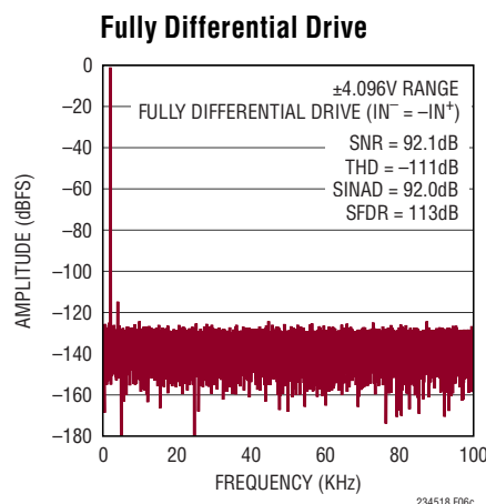
Figure 6c. IN^+/IN^- = -1dBFS 2kHz Fully Differential Sine, Common Mode = 2.5V, 32k Point FFT, f_{SAMPL} = 200ksps . Circuit Shown in Figure 6a with LT6237 Amplifiers, R_{FILT} = 40.2\Omega , C_{FILT} = 1nF
