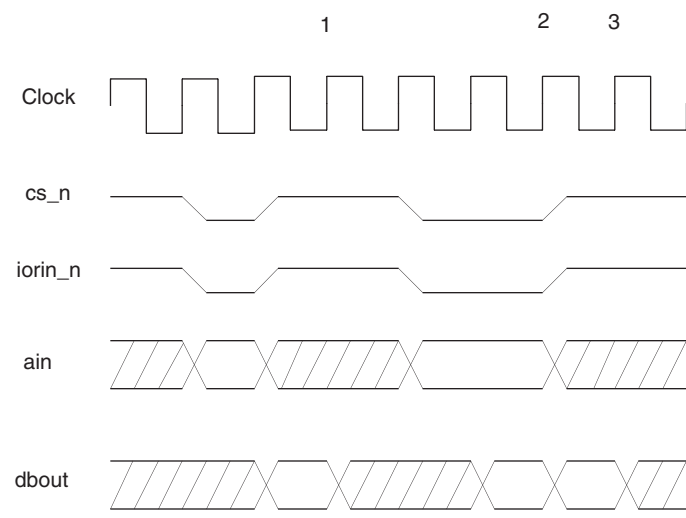
Figure 4. Processor Read Timing Waveform
