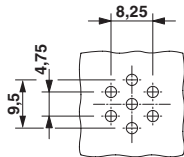
Drilling diagram
