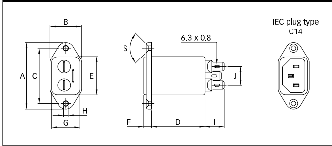
FN 9222 1 to 15 A types
