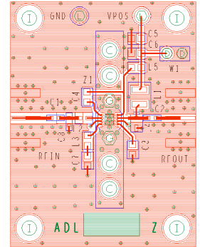
Figure 18. Evaluation Board Layout (Top)
