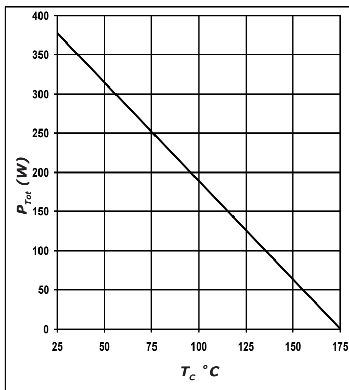
Figure 4. Power Derating
