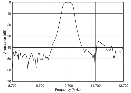
SFECF10M7EA00S0-R0
