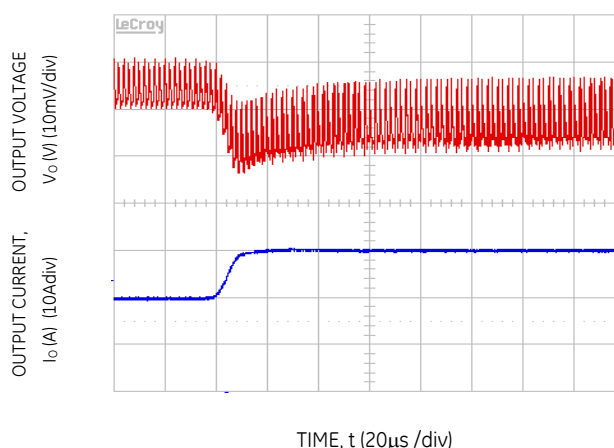
Figure 4. Transient Response to Dynamic Load Change from 50% to 100% at 12Vin, C out = 1x47μF + 11x330μF CTune=47nF, RTune=178 ohms
