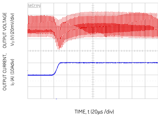
Figure 10. Transient Response to Dynamic Load Change from 50% to 100% at 12Vin, Cout= 1x47uF +5x330uF, CTune=10nF & RTune=178 ohms
