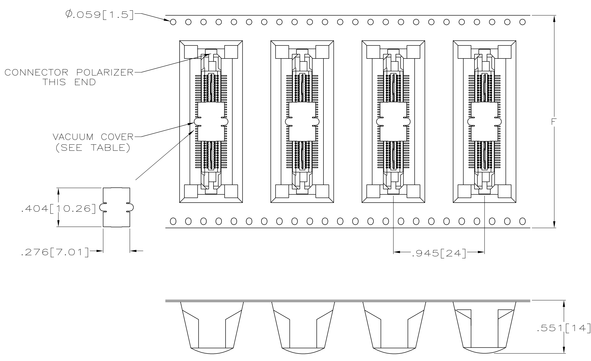
PACKAGING DETAIL SCALE 2:1 DIMENSIONS ARE FOR REFERENCE
