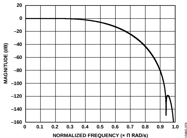
Figure 107. HB4 Filter Response
