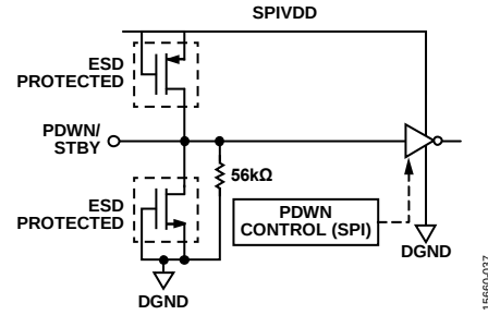
Figure 65. PDWN/STBY Input
