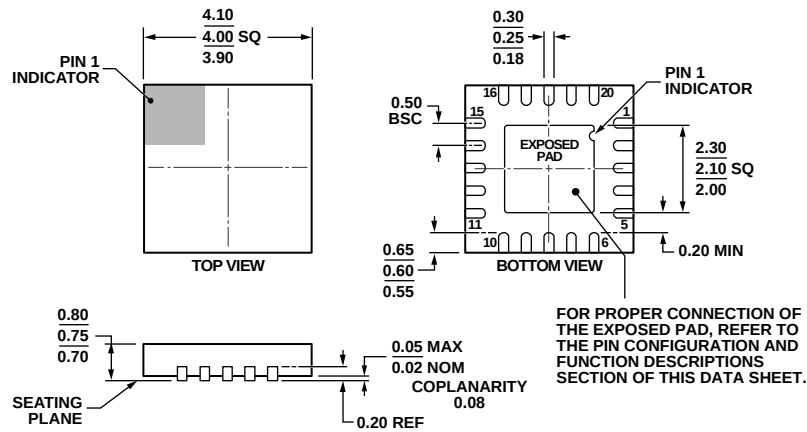
Figure 61. 20-Lead Lead Frame Chip Scale Package [LFCSP_WQ] 4 mm x 4 mm Body, Very Thin Quad (CP-20-6) Dimensions shown in millimeters
