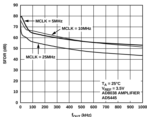
Figure 37. Wideband SFDR vs. f_{OUT} Frequency
