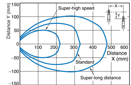
Through-beam E32-T14LR
