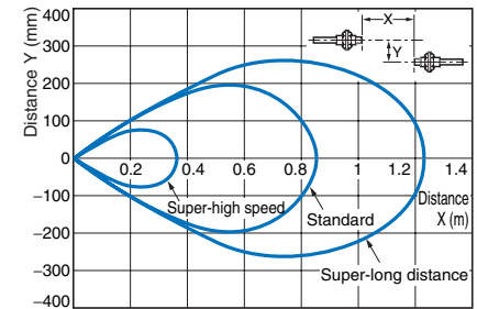
Through-beam E32-T22R
