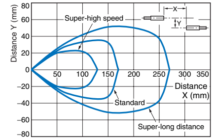
Through-beam E32-T14LR
