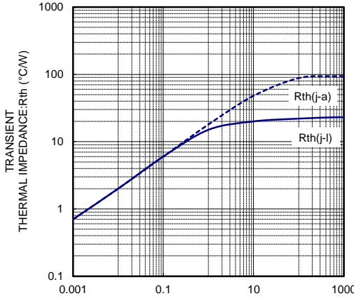
R_th-t CHARACTERISTICS
