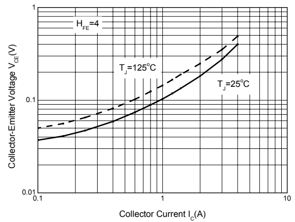
Figure 9. Collector-Emitter Saturation Region
