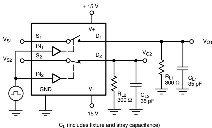
Figure 2. Break-Before-Make (DG456)
