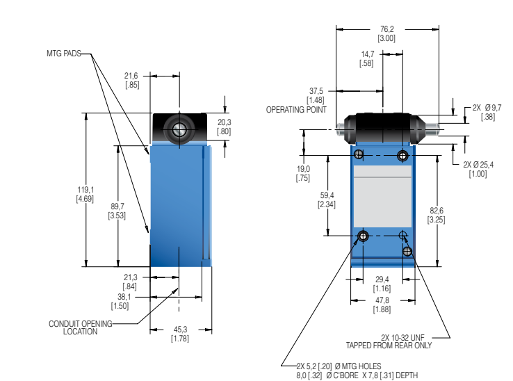
DPDT Non-plug-in (mm[in])
