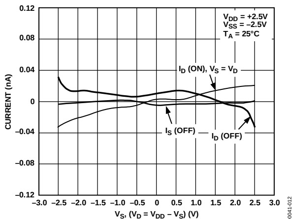
Figure 12. Leakage Currents as a Function of V_D ( V_S = V_D )
