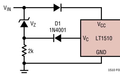
Figure 3. Undervoltage Lockout
