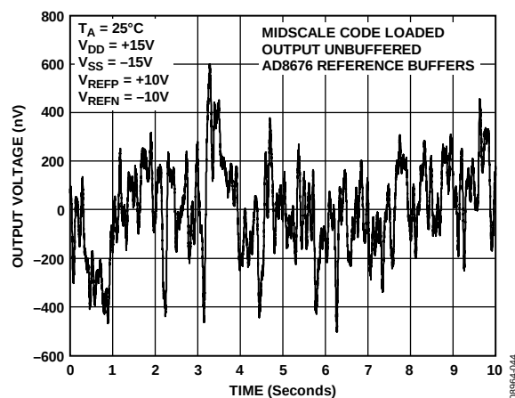
Figure 46. Voltage Output Noise, 0.1 Hz to 10 Hz Bandwidth
