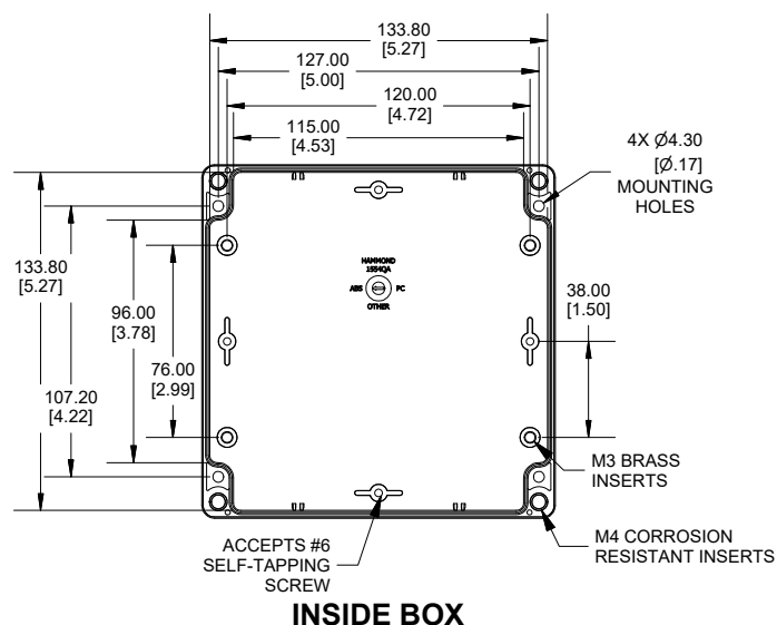
INSIDE BOX
