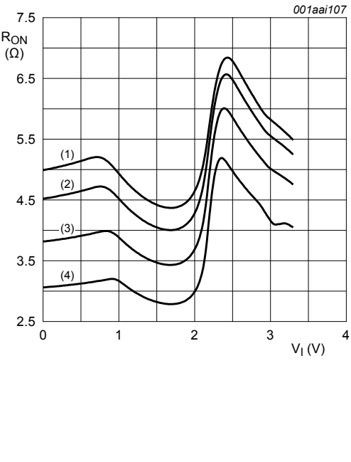
Fig. 14. ON resistance as a function of input voltage; V_{CC} = 3.3\text{ V} ; I_{SW} = 64\text{ mA}
