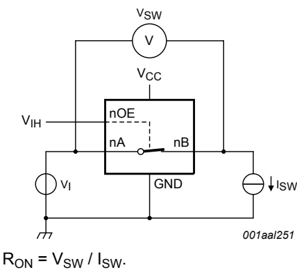
Fig. 8. Test circuit for measuring ON resistance (one switch)
