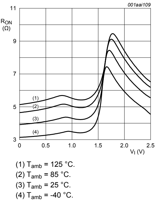
Fig. 9. ON resistance as a function of input voltage; V_{CC} = 2.5\text{ V} ; I_{SW} = 15\text{ mA}
