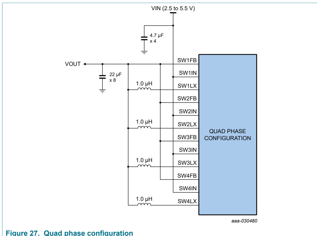
Figure 27. Quad phase configuration
