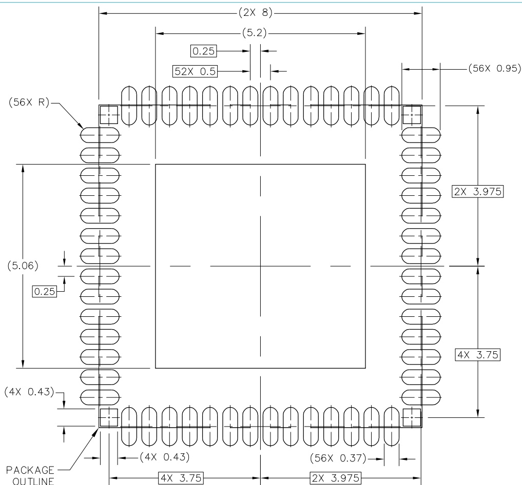
Figure 45. Solder mask pattern
