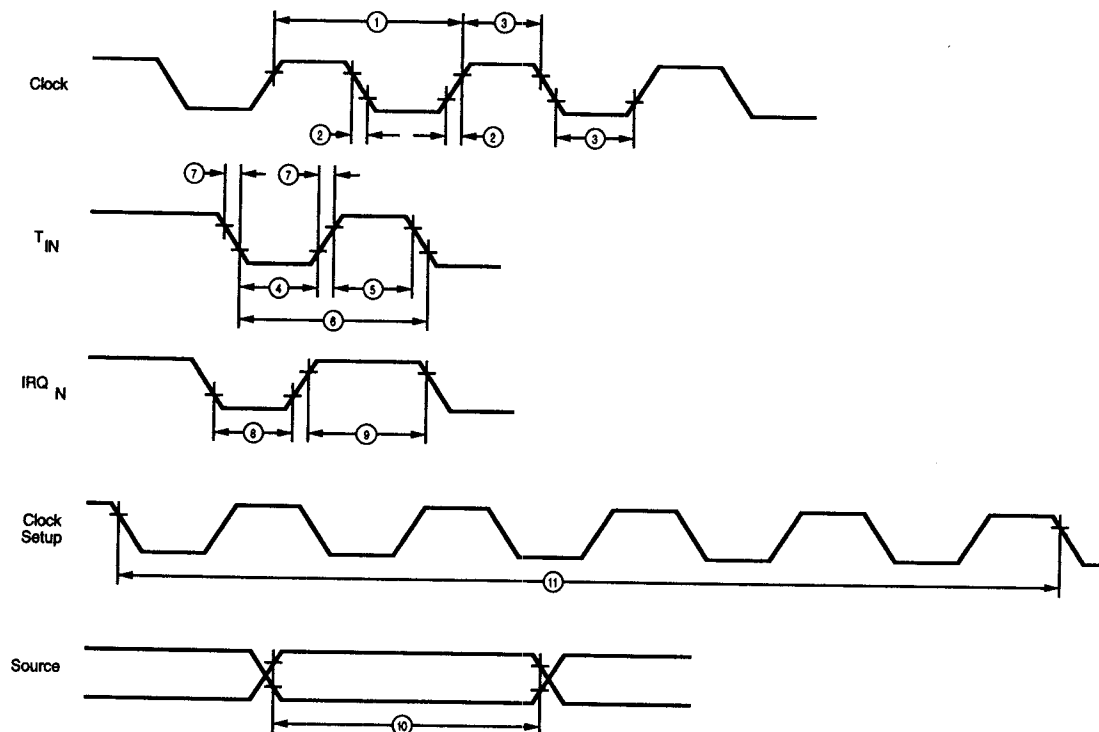
Figure 29. Additional Timing
