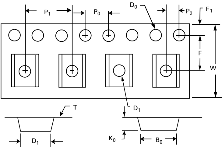
Tape Specifications
