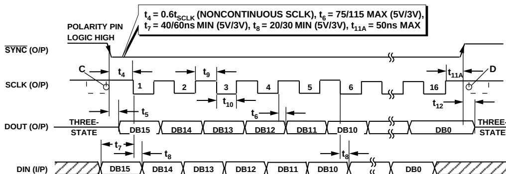
Figure 39. Timing Diagram for Read/Write with \overline{SYNC} Output and \overline{SCLK} Output (Continuous and Noncontinuous) (i.e., Operating Mode Numbers 4 and 5, SM1 = 1 , SM2 = 1 and 0)
