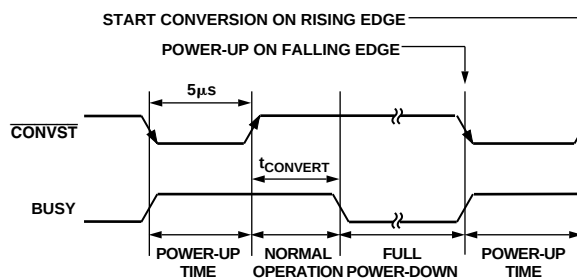
Figure 24. Power-Up Timing When Using CONVST Pin
