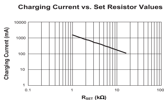
Figure 2: Constant Charging Current vs. Set Resistor Values.
