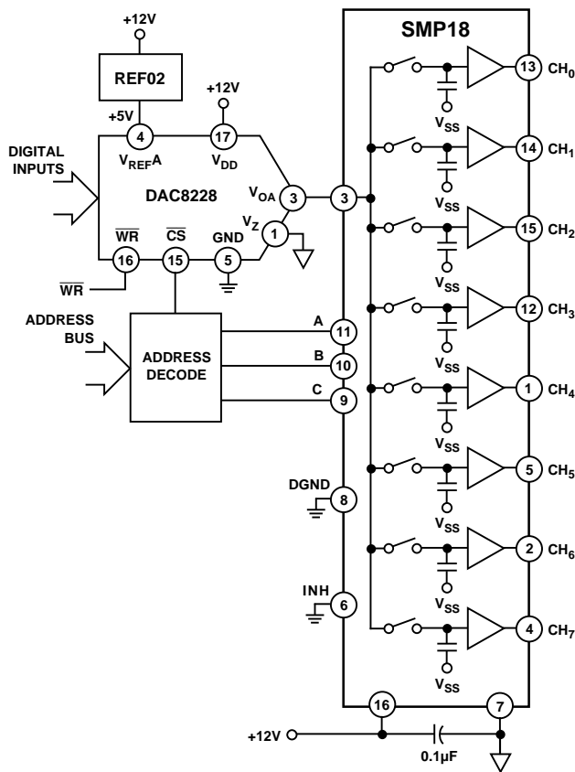
Figure 1. 8-Channel Multiplexed D/A Converter
