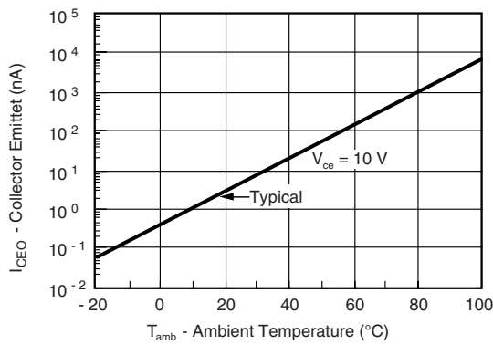
Fig. 16 - Collector Emitter Leakage vs. Temperature
