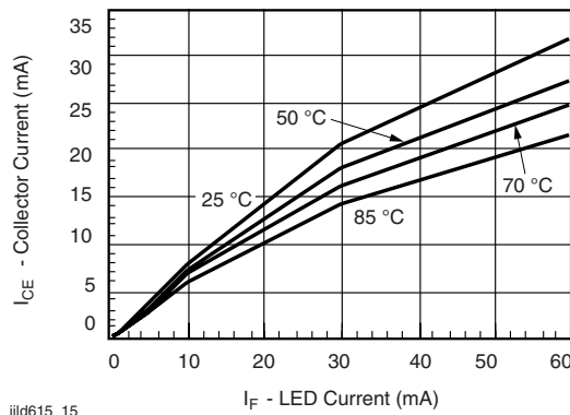
Fig. 15 - Collector Emitter Current vs. Temperature and LED Current
