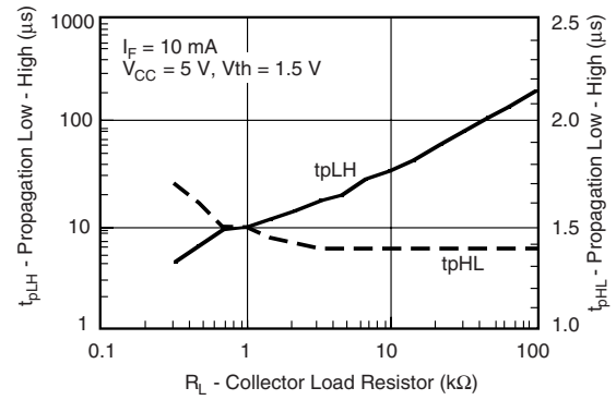
Fig. 19 - -4, Propagation Delay vs. Collector Load Resistor
