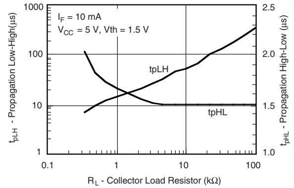
Fig. 18 - -2, -3, Propagation Delay vs. Collector Load Resistor
