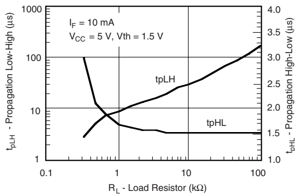
Fig. 17 - -1, Propagation Delay vs. Collector Load Resistor
