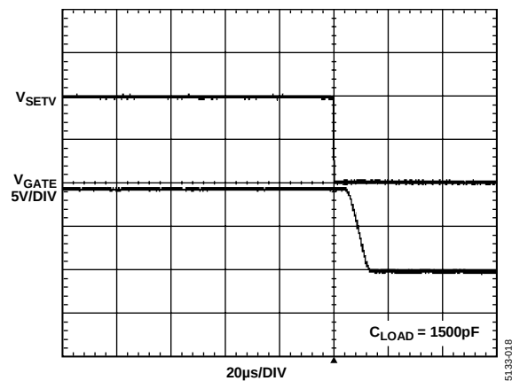
Figure 16. Gate Turn-Off Time
