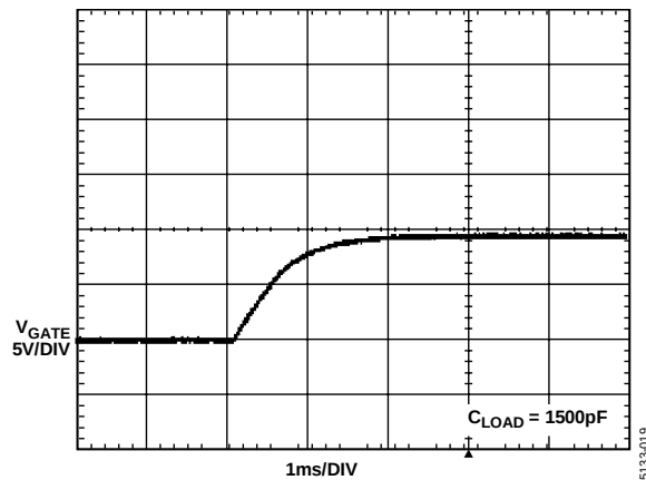
Figure 17. Gate Turn-On Time
