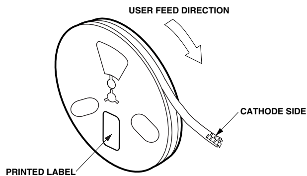
Figure 14. Reeling orientation
