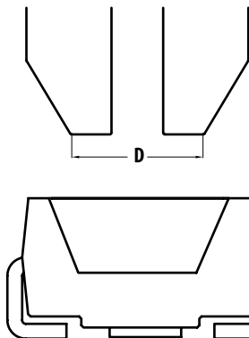
Figure 11. Recommended Pick and Place Nozzle Size for InGaN Family
