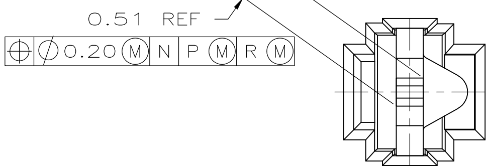
VIEW W-W SCALE 20:1
