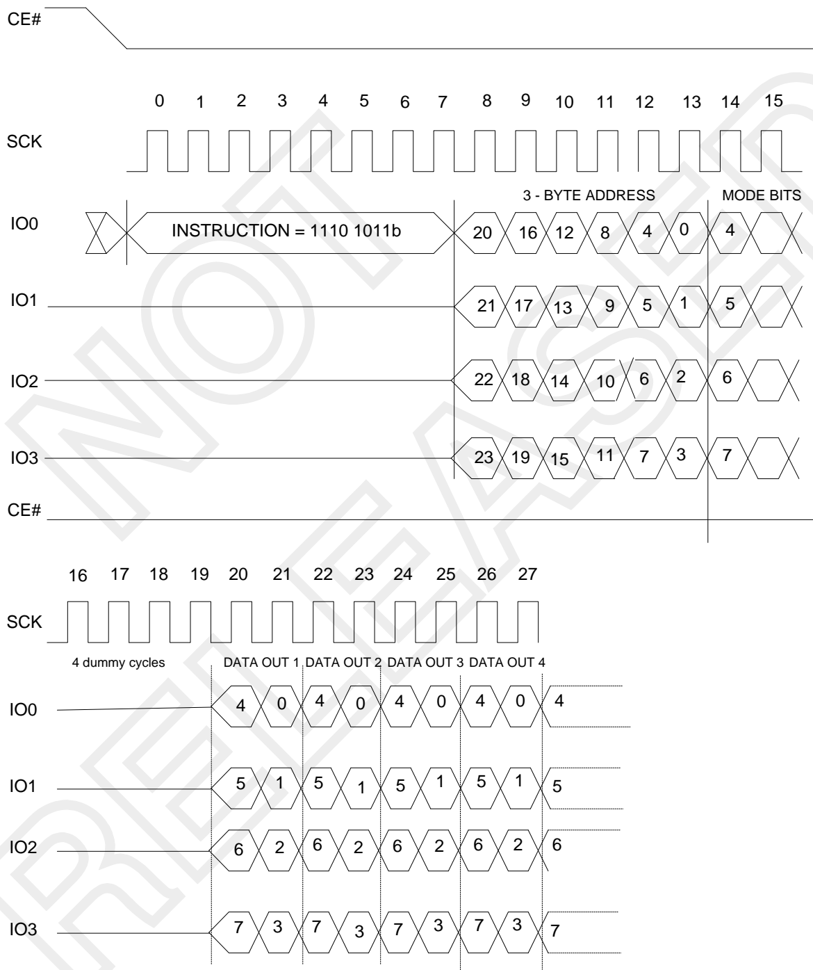
Figure 18. Fast Read Quad I/O Sequence (with command decode cycles)
