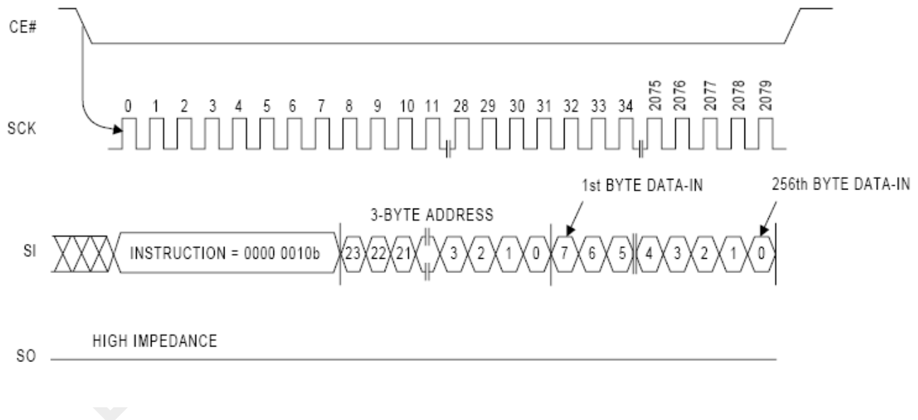
Figure 21. Page Program Sequence
