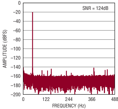
32k Point FFT f_{SAMPL} = 1\text{Mps} , f_{IN} = 50\text{Hz} , N = 1024
