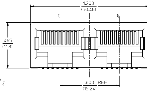
8 CIRCUIT ASSEMBLY
