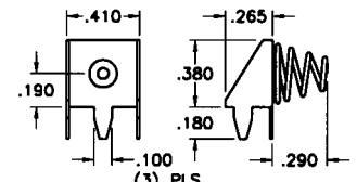
Mounting Detail
