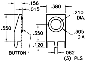
Mounting Detail
